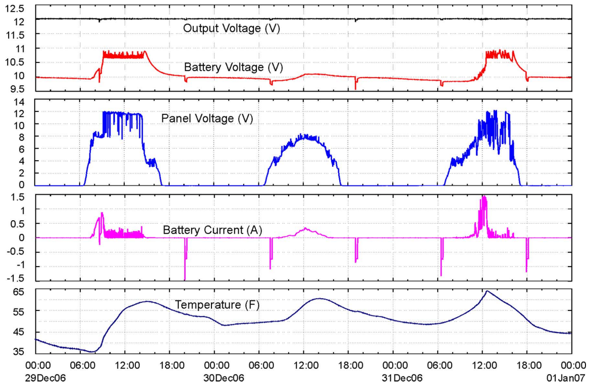
Fig. 12. Data from deployed demonstration unit in Champaign, IL.
