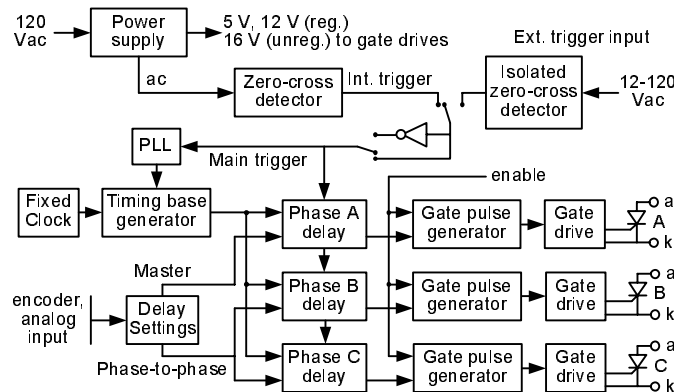
Fig 2. SCR box system block diagram.
