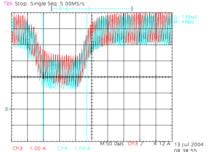
Figure 5: Inductor Current Waveforms Through Load Transient
