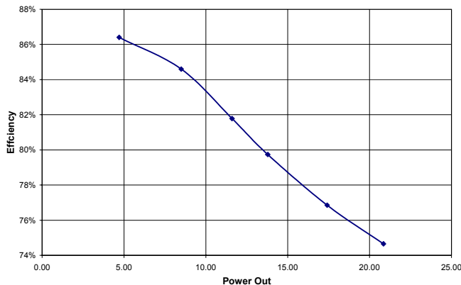
Figure 6: SIPO Efficiency
