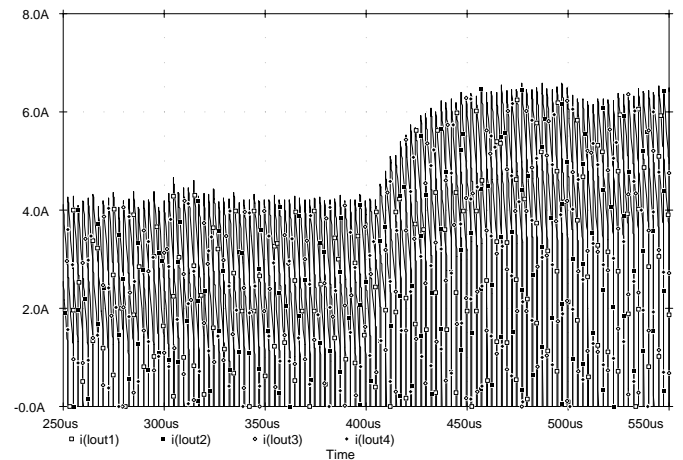
Figure 3: Output Currents, Four Stages of Fig. 1
