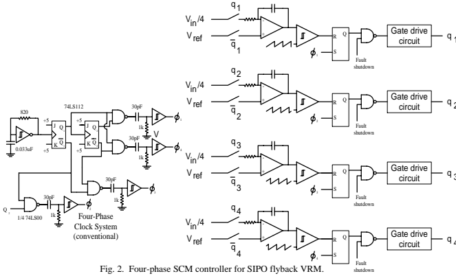
Fig. 2. Four-phase SCM controller for SIPO flyback VRM.
