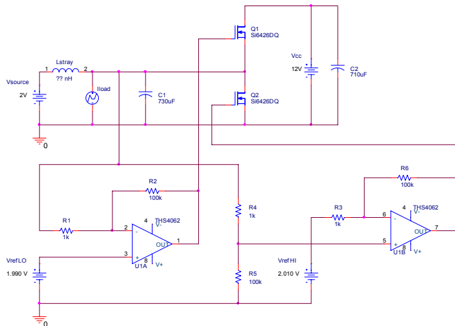
Figure 7: Simplified Active Clamp Circuit
